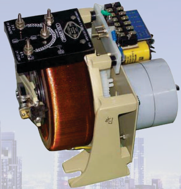
Single Phase Open Motorized Variac Dimmer
